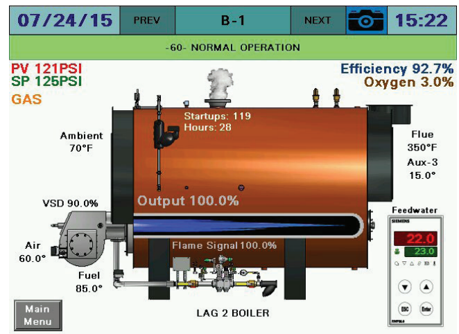
Boiler Overview Screen
